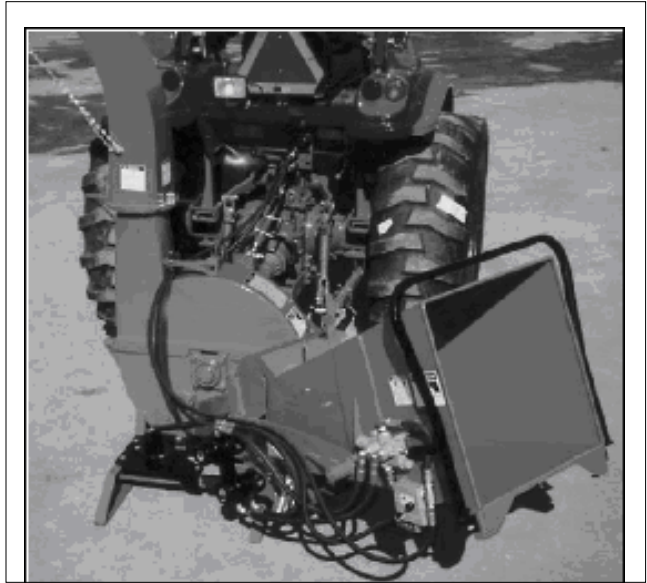
Fig. 30 CLEANING
