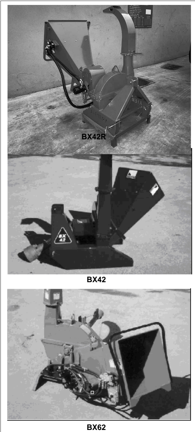
Fig. 43 MACHINE
