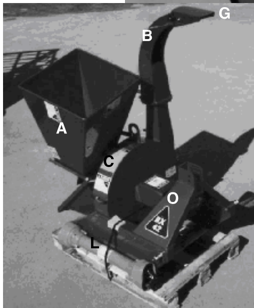
Fig. 10 PRINCIPLE COMPONENTS
